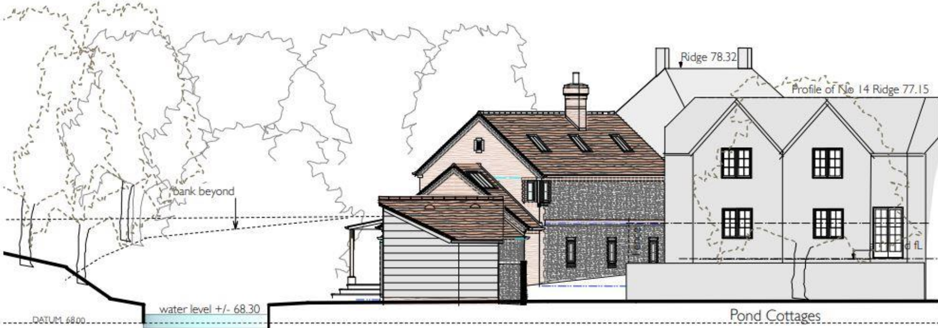
3. EAST ELEVATION
